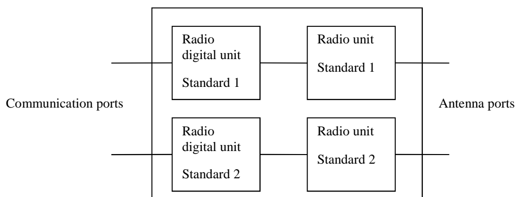
Figure 1: Multi-radio equipment
