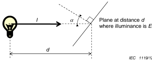
Figure 6 – Relation of illuminance E , distance d and intensity I
